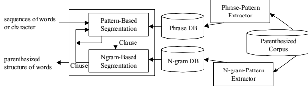
Fig.2 The Architecture of NL Parser
